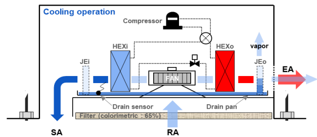
Drain-less system
