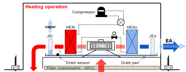
Drain-less system
